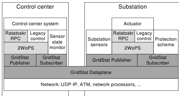
Figure 2. Ratoskr module stack
